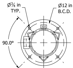
BASE BOLT PATTERN
