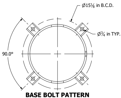
BASE BOLT PATTERN
