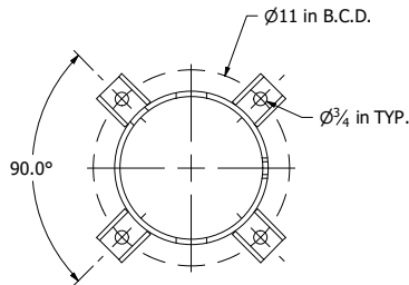
BASE BOLT PATTERN
