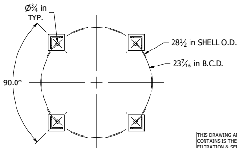
BASE BOLT PATTERN
